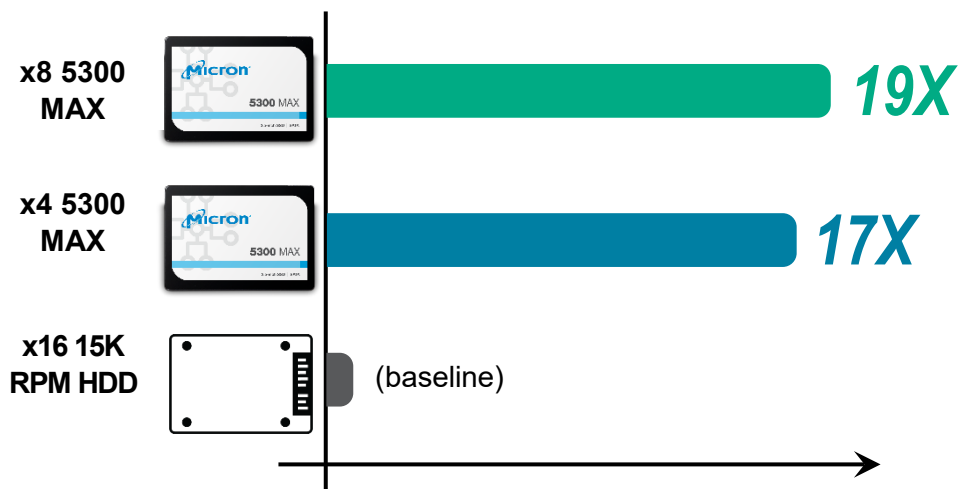
Figure 3: Power Efficiency
